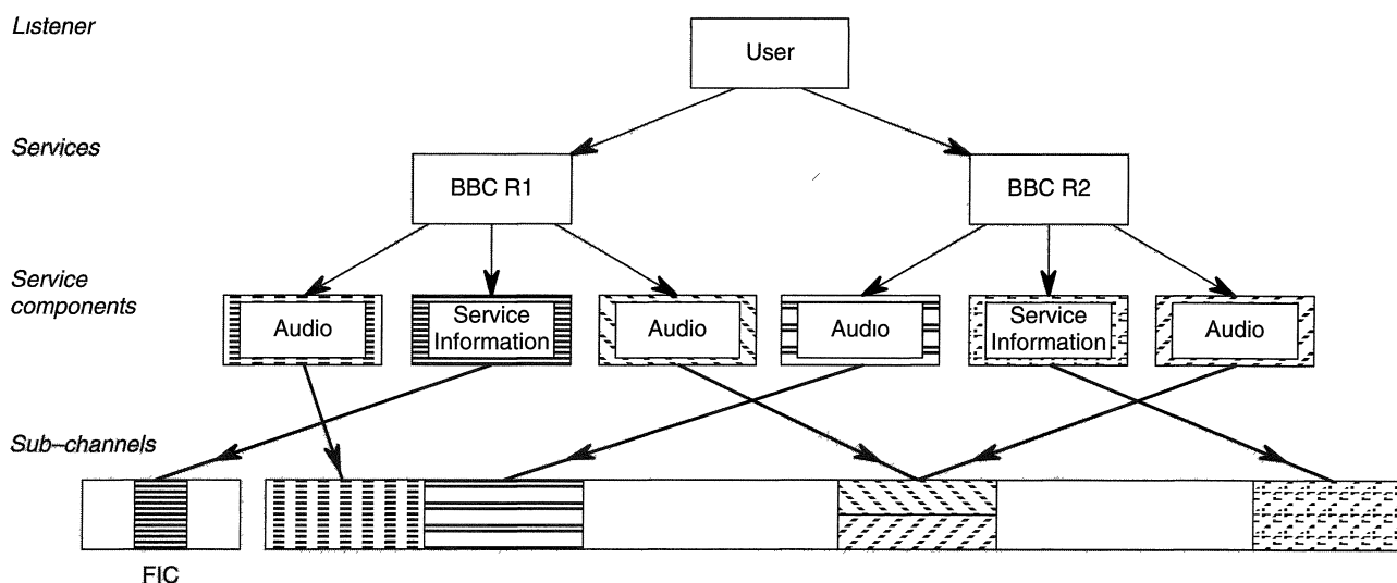
Figure 3 DAB service structure.
